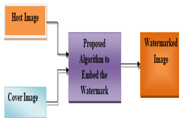
Fig.1.Basic Watermarking Principle
